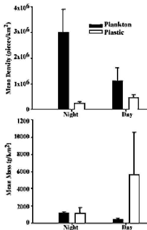
FIGURE 2. Abundance and mass of plankton and plastic in night versus day samples.
